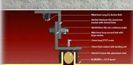
CLADDING TO CLADDING INTERFACE
