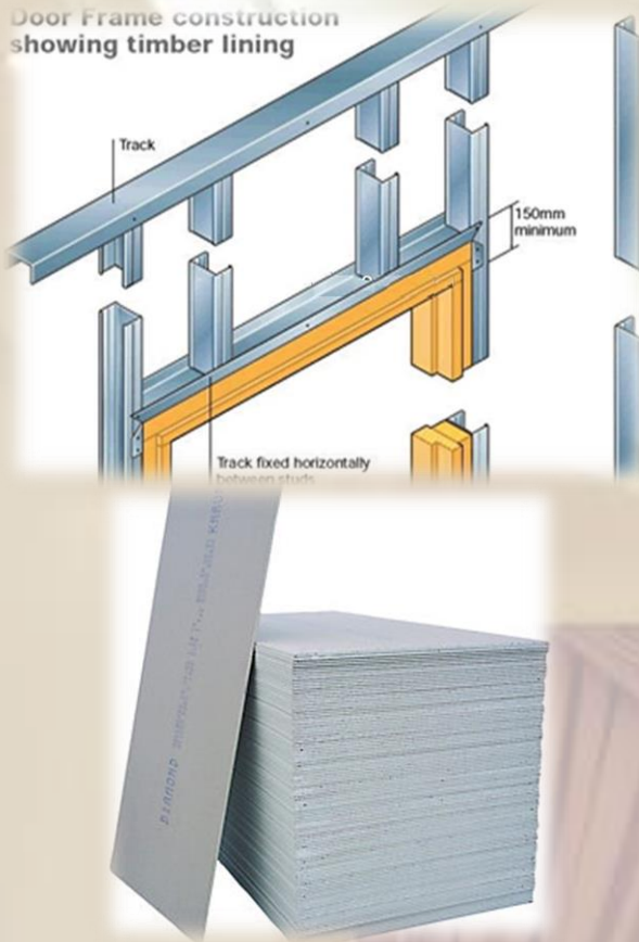
100mm Thick HDP Drywall Partition System
