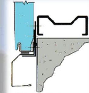
24 DRIP - Horizontally laid panels
