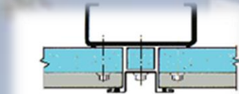
28 VERTICAL JOINT - Horizontally laid panels
