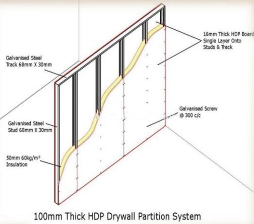
100mm Thick HDP Drywall Partition System
