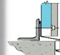
24 DRIP - Horizontally laid panels
