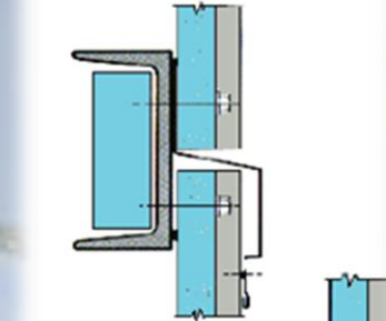
29 HORIZONTAL JOINT - Vertically laid panels
