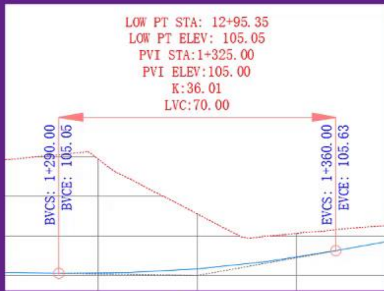
Sag Curve
