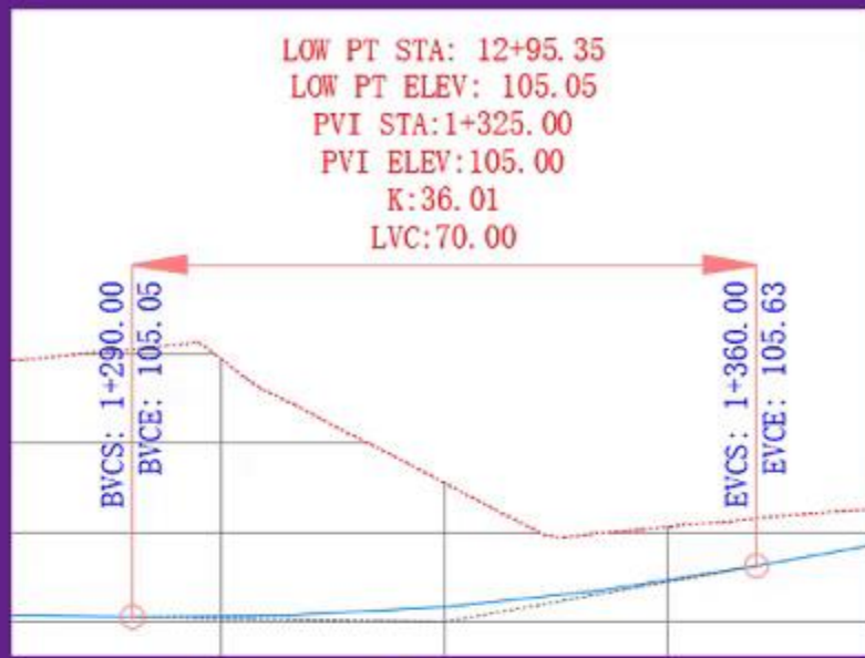
Sag Curve
