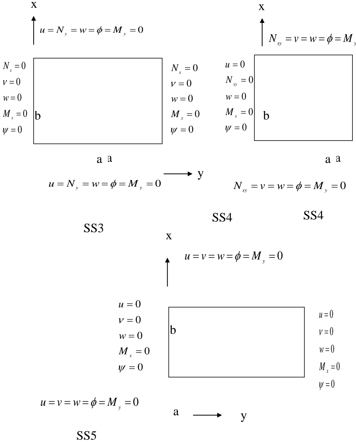
Fig. (1) Simply supported boundary conditions
